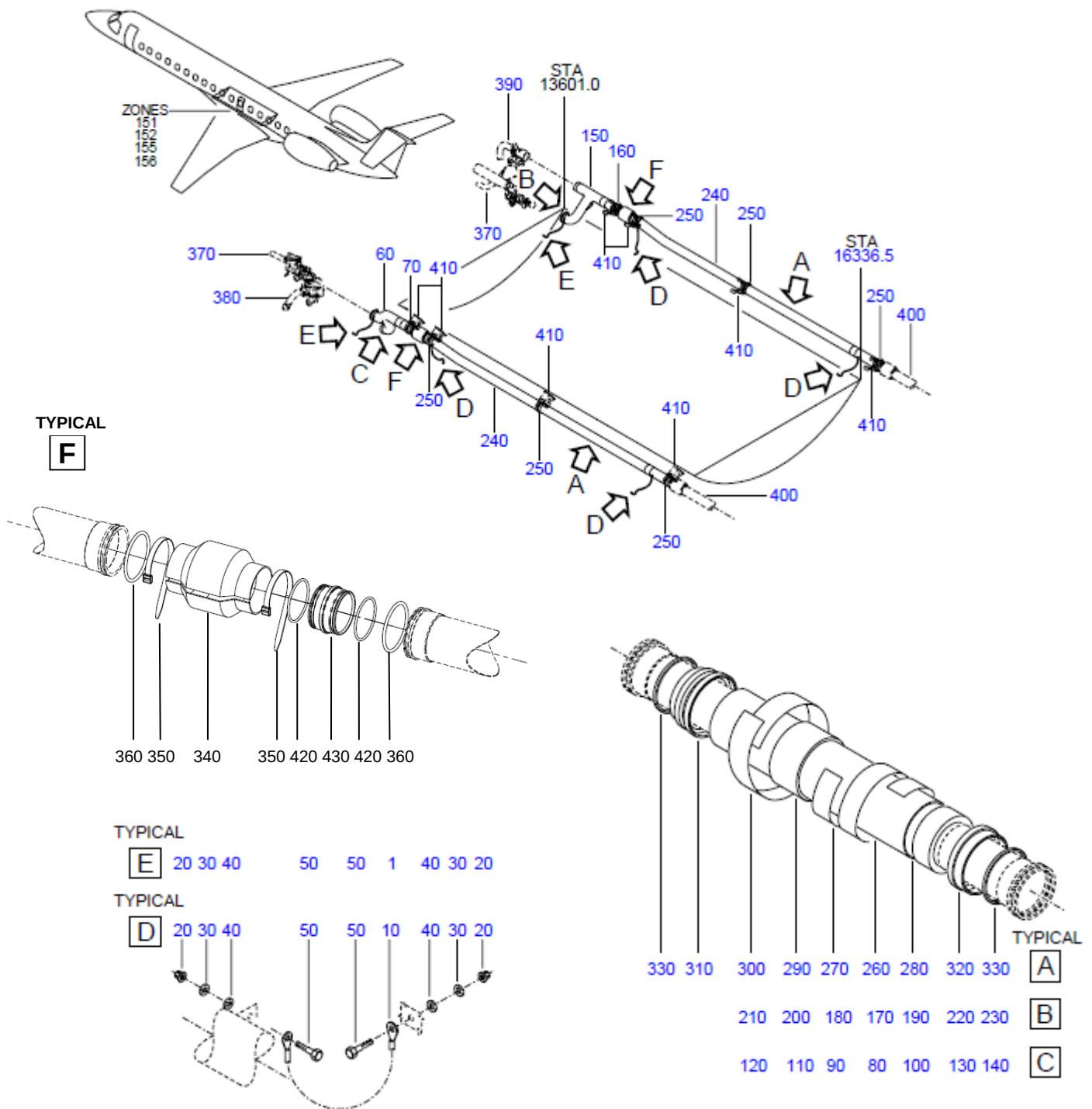
FIGURE 01(SUP) - ENGINE BLEED AIR SYS INSTL, BTW FR 40 AND FR 49
