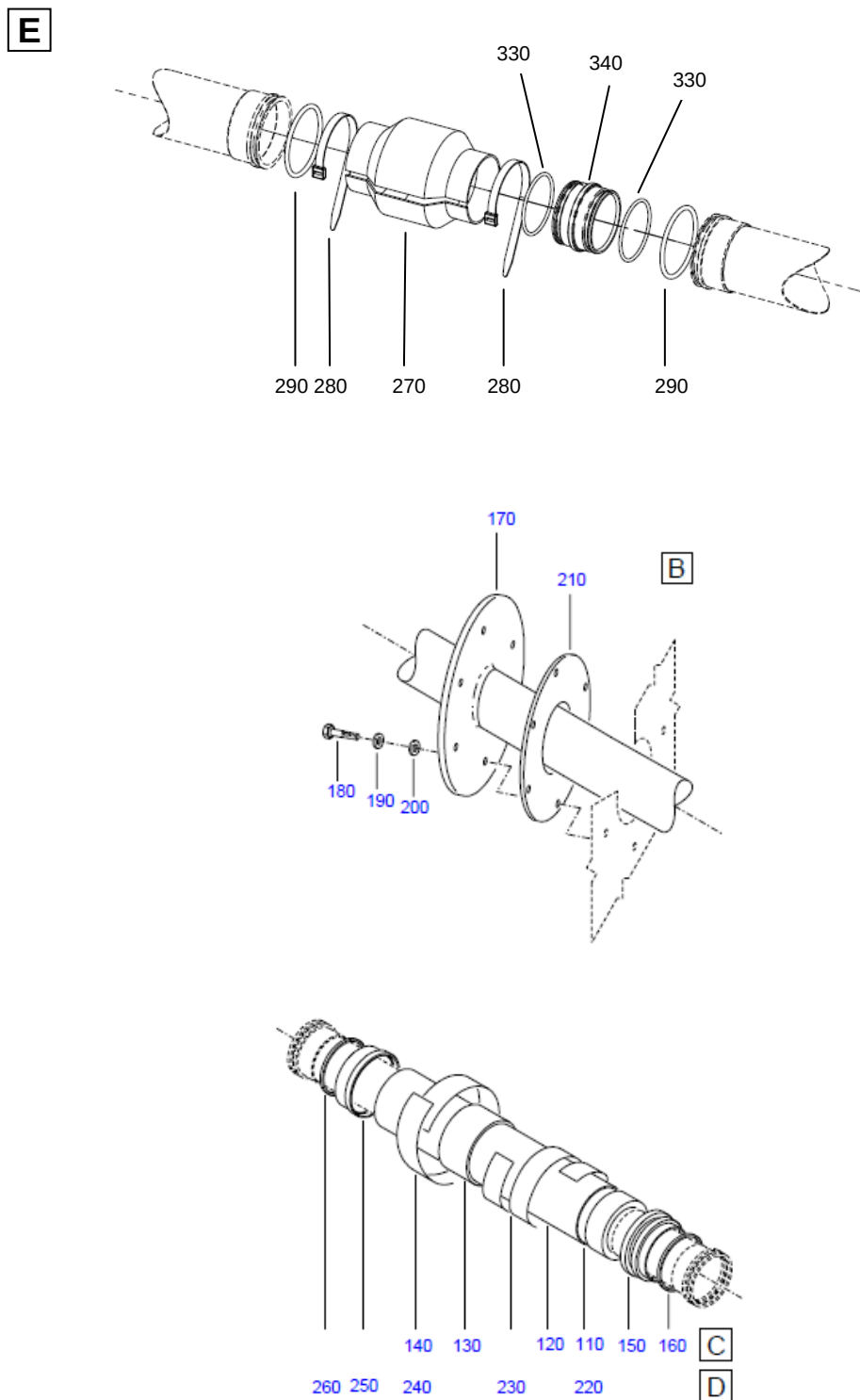
FIGURE 03(SUP) - ENGINE BLEED AIR SYS INSTL, BTW FR 74 AND FR 76 Sheet 2 of 2
