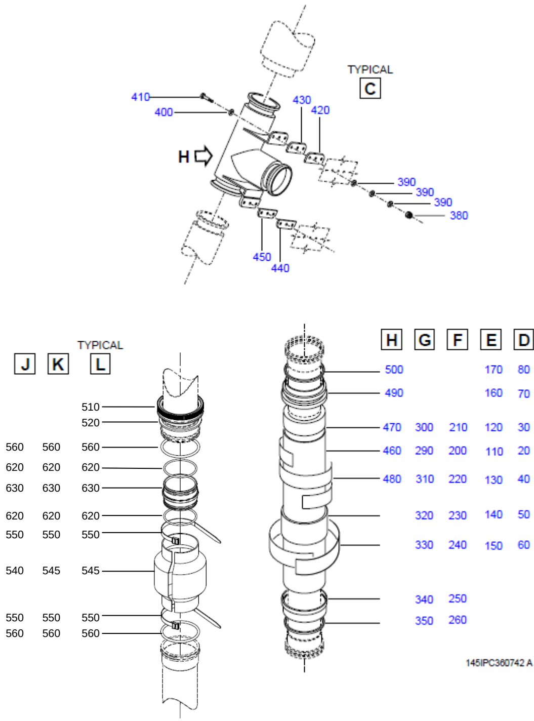
FIGURE 20(SUP) - ENGINE BLEED AIR SYS INSTL, FR 69 Sheet 2 of 2
