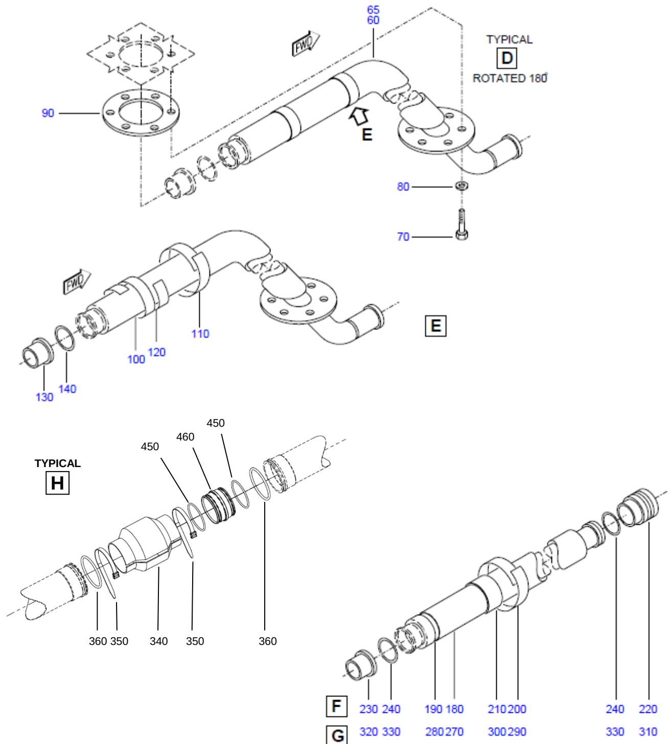
FIGURE 22(SUP) - ENGINE BLEED AIR SYS INSTL, BTW FR 55 AND FR 60 Sheet 2 of 2
