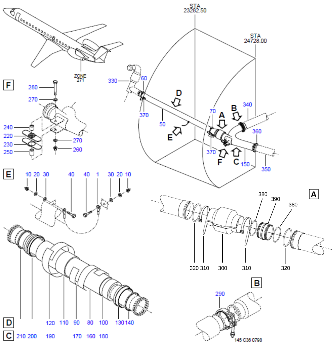
FIGURE 41(SUP) - ENGINE BLEED AIR SYS INSTL, BTW FR 70 AND FR 74, LH SIDE
