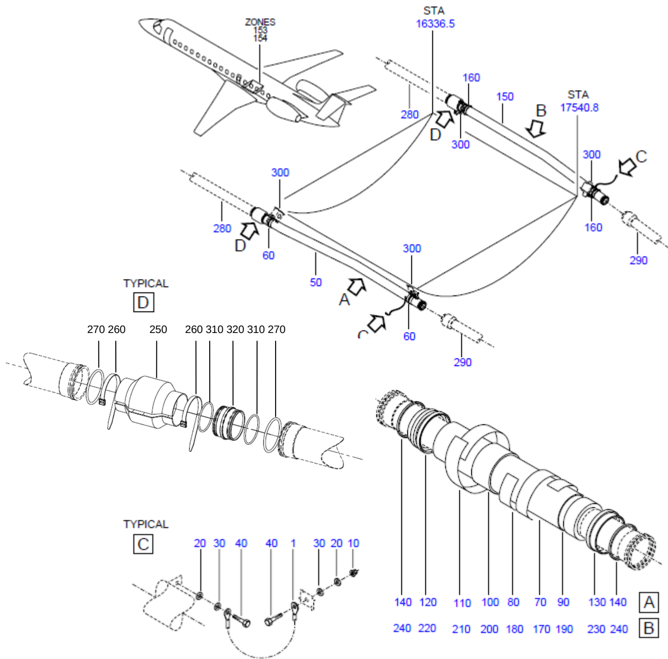
FIGURE 20(SUP) - ENGINE BLEED AIR SYS INSTL, BTW FR 49 AND FR 52
