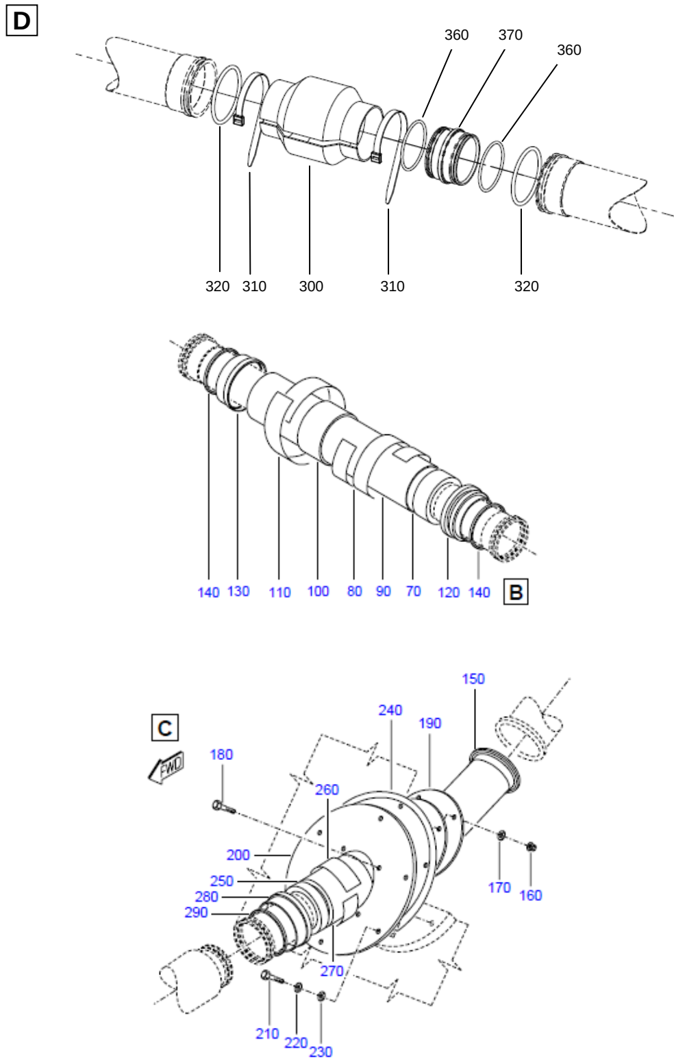
FIGURE 10(SUP) - ENGINE BLEED AIR SYS INSTL, BTW FR 76 AND FR 80 Sheet 2 of 2
