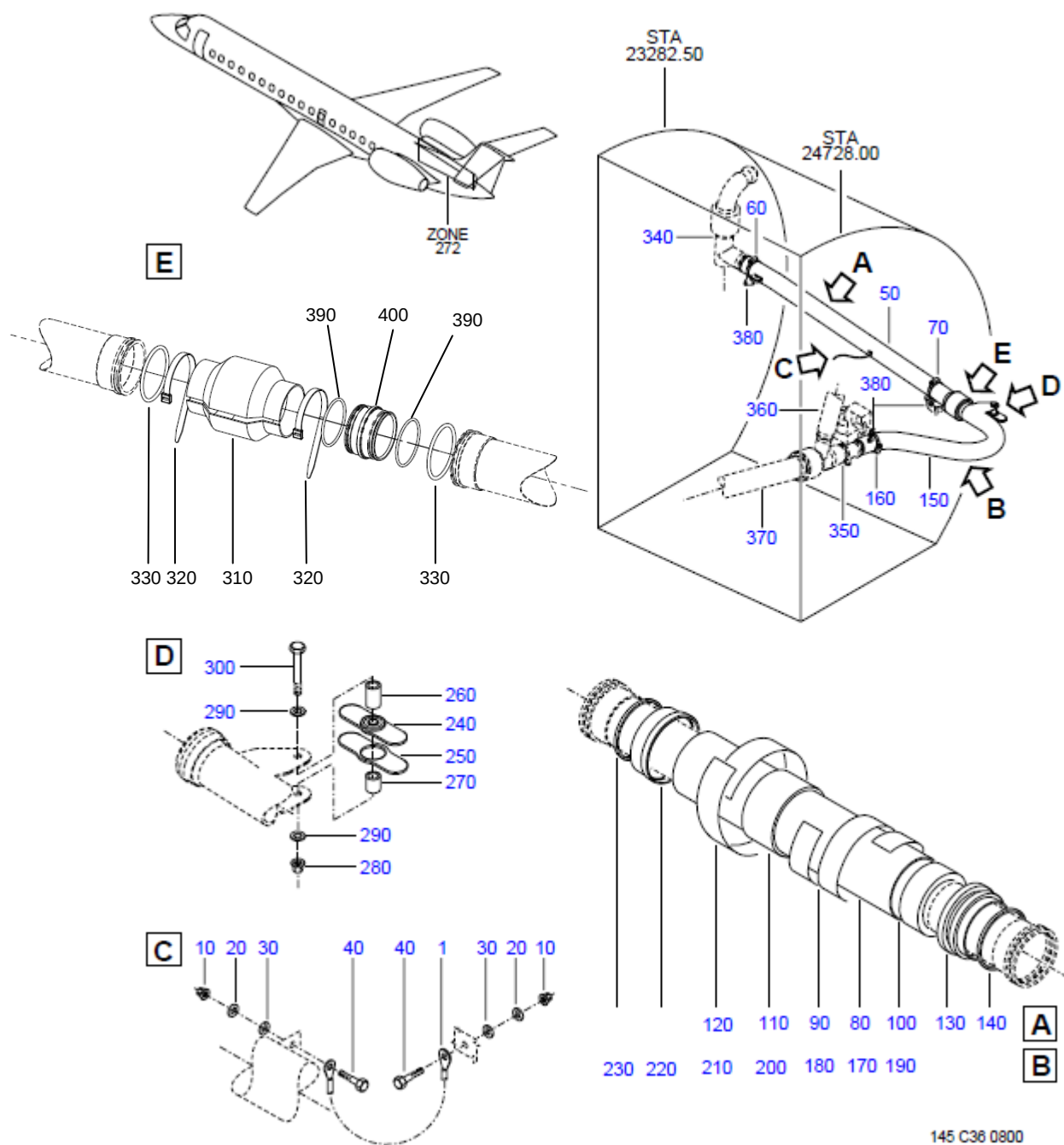
FIGURE 51(SUP) - ENGINE BLEED AIR SYS INSTL, BTW FR 70 AND FR 74, RH SIDE
