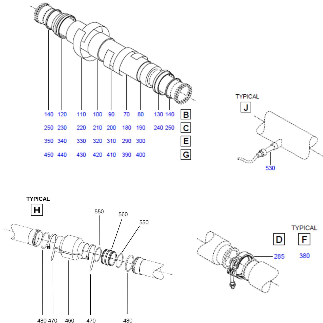
FIGURE 02(SUP) - ENGINE BLEED AIR SYS INSTL, BTW FR 60 AND FR 70 Sheet 2 of 2
