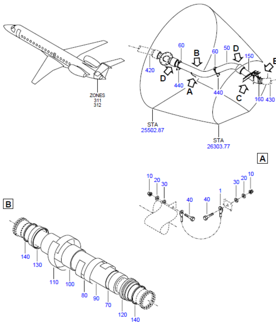
FIGURE 11(SUP) - ENGINE BLEED AIR SYS INSTL, BTW FR 76 AND FR 80 Sheet 1 of 2
