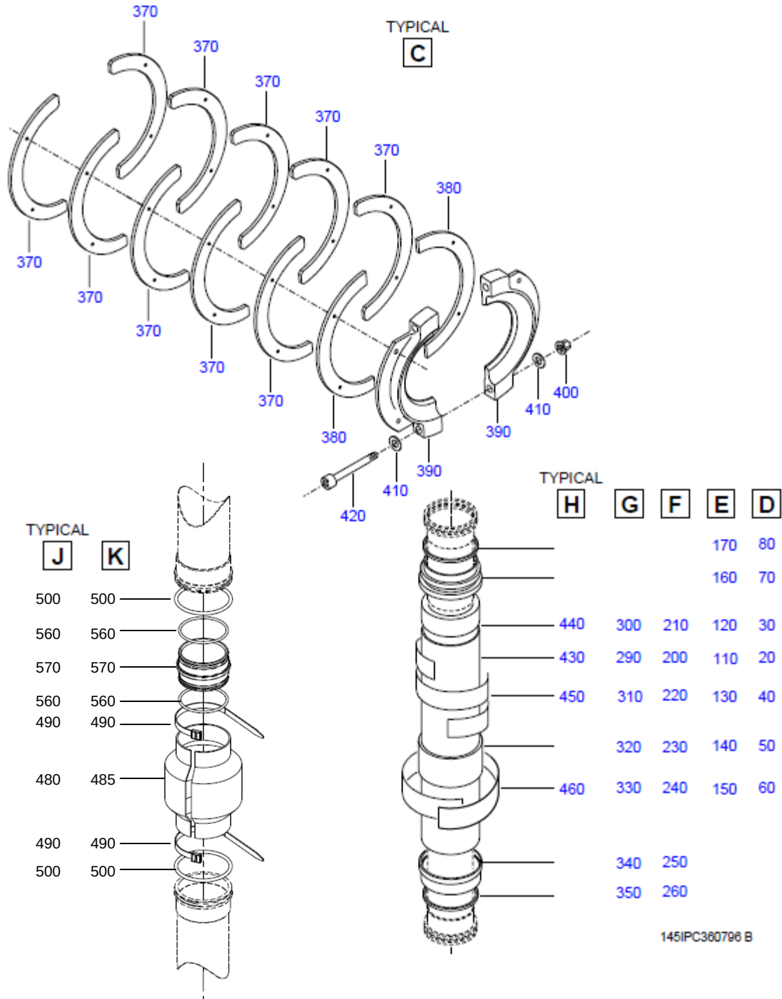
FIGURE 21(SUP) - ENGINE BLEED AIR SYS INSTL, FR 69 Sheet 2 of 2
