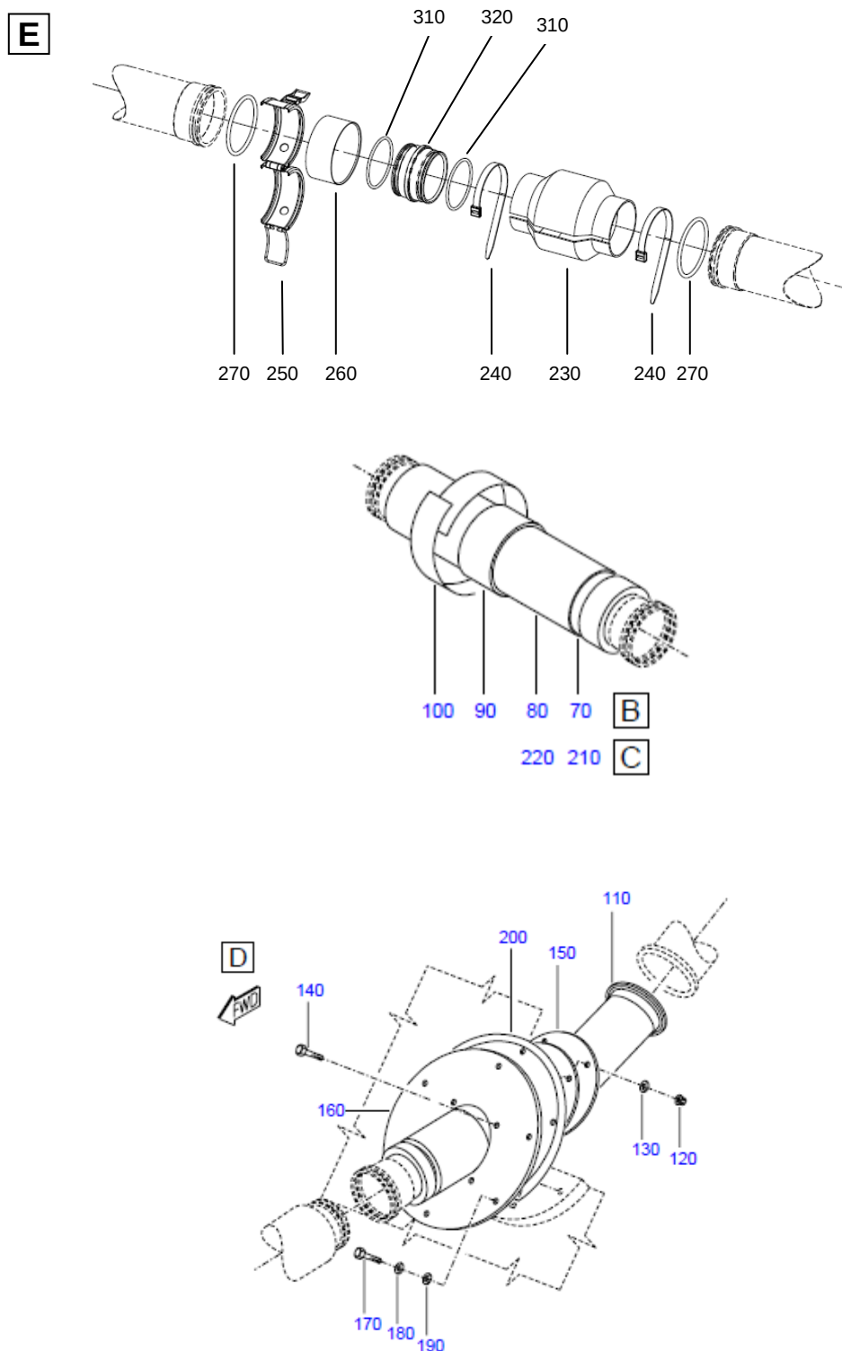
FIGURE 11(SUP) - ENGINE BLEED AIR SYS INSTL, BTW FR 76 AND FR 80 Sheet 2 of 2
