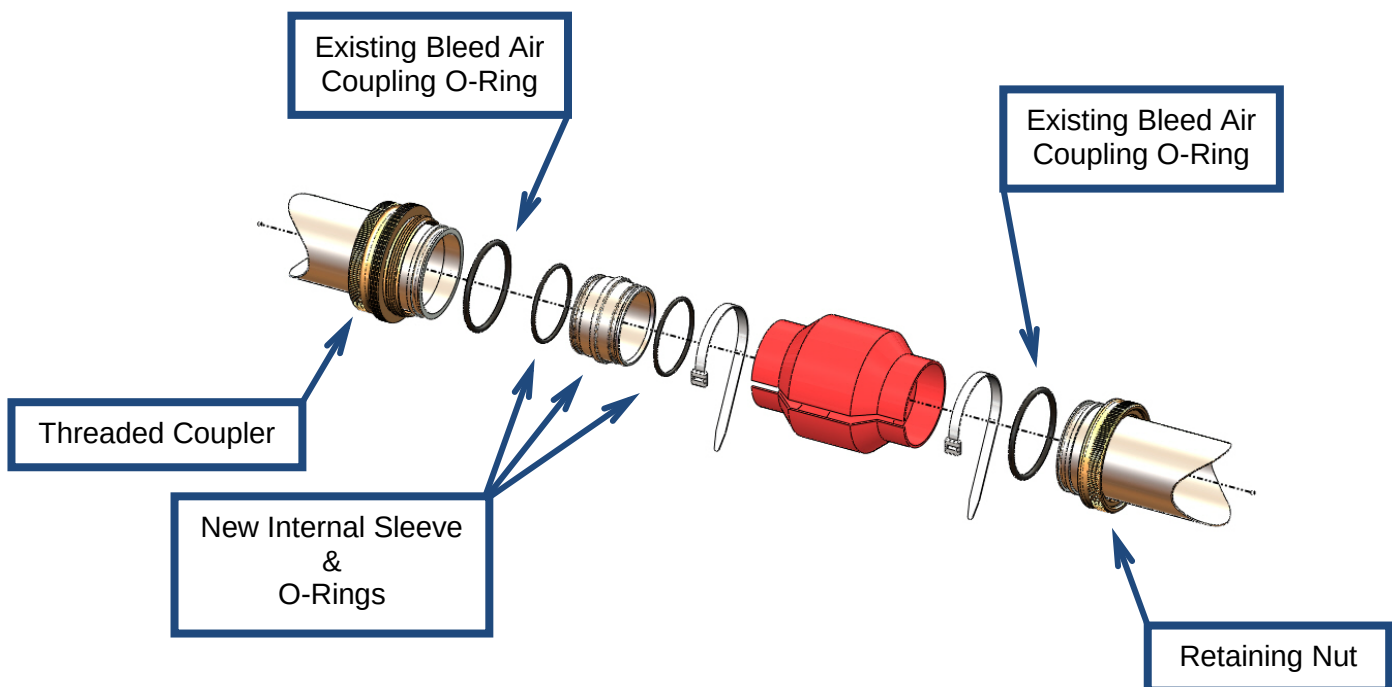
Figure 1 Bleed Air Duct Coupling Flanged Design with Threaded Coupler & Retaining Nut
