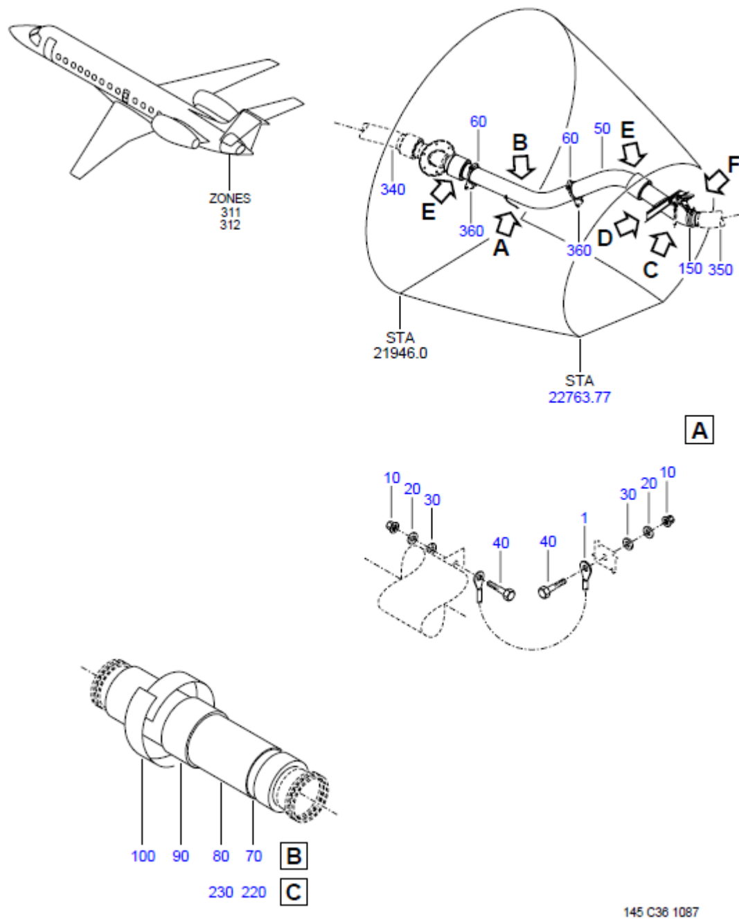
FIGURE 11A(SUP) - ENGINE BLEED AIR SYS INSTL, BTW FR 76 AND FR 80 Sheet 1 of 2
