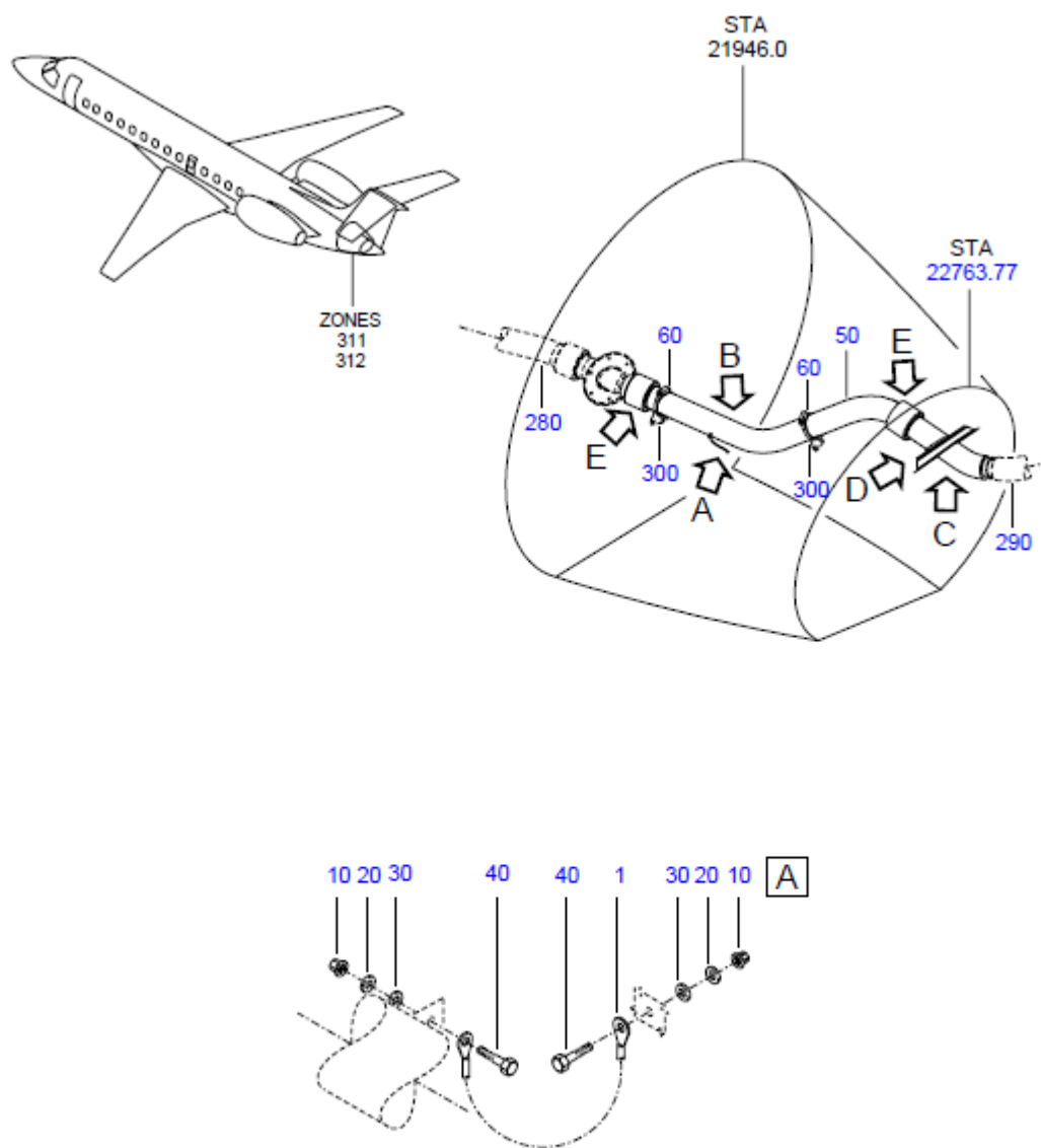
FIGURE 11(SUP) - ENGINE BLEED AIR SYS INSTL, BTW FR 76 AND FR 80 Sheet 1 of 2
