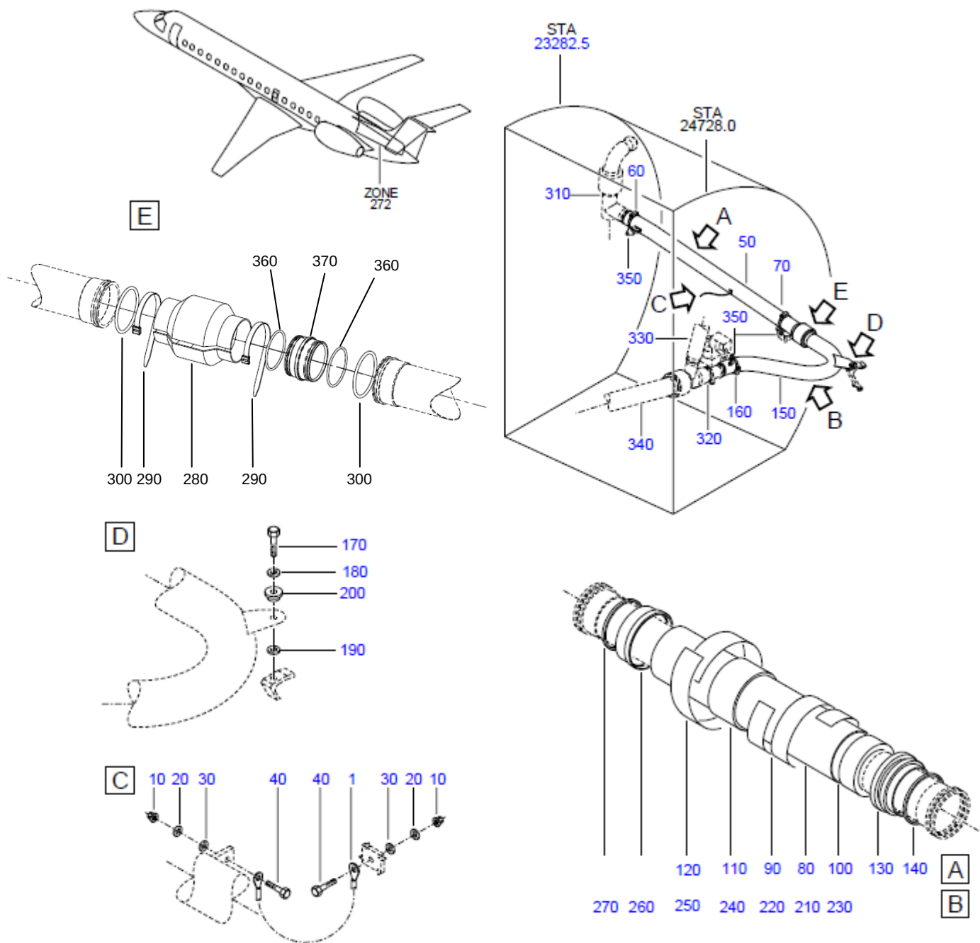
FIGURE 50(SUP) - ENGINE BLEED AIR SYS INSTL, BTW FR 70 AND FR 74, RH SIDE
