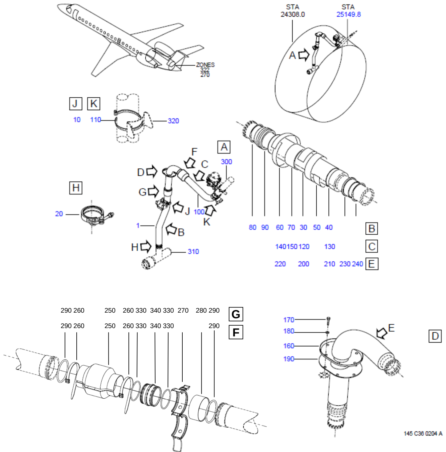
FIGURE 21(SUP) - ENGINE BLEED AIR SYS INSTL, BTW FR 73 AND FR 75
