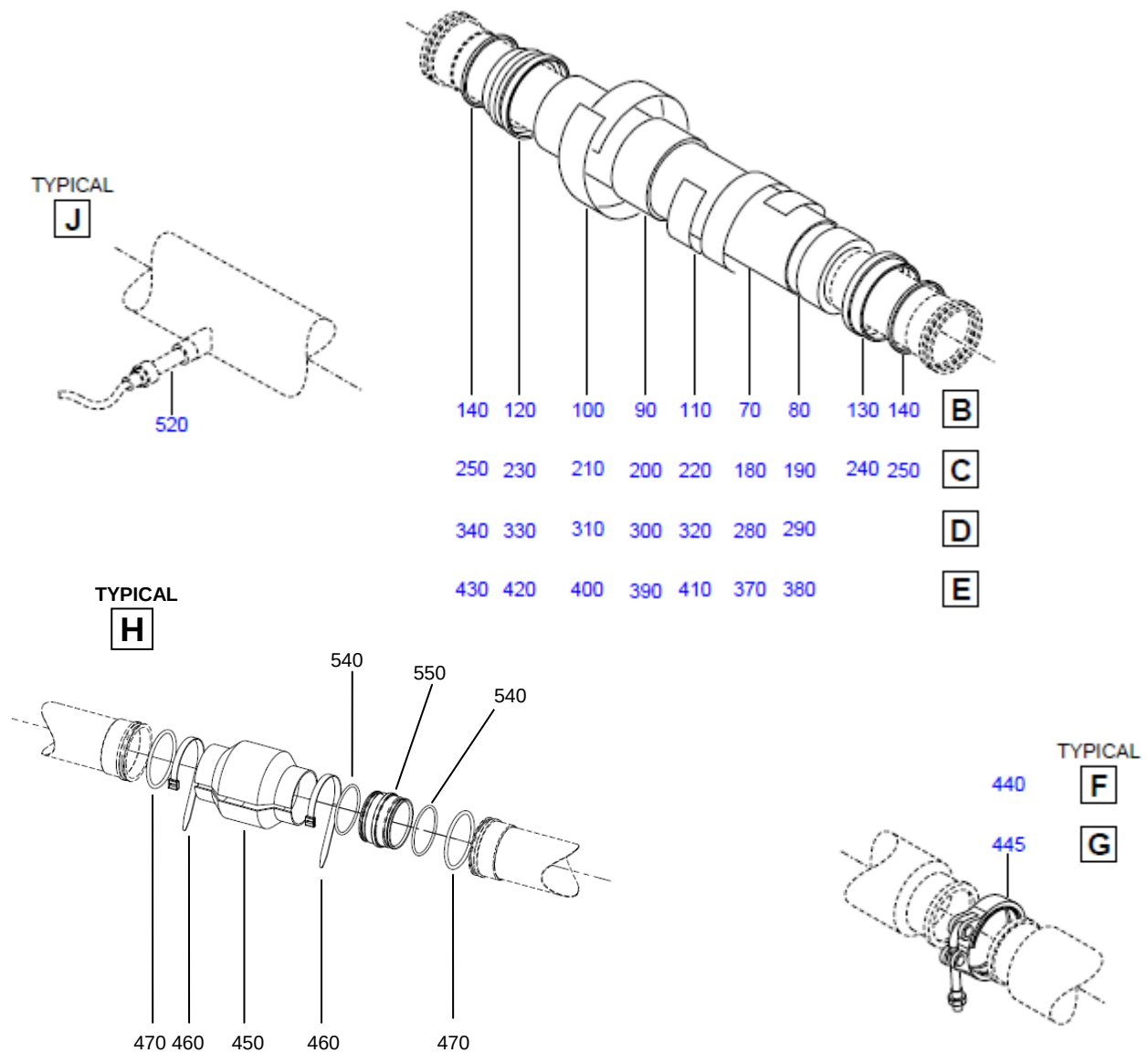
FIGURE 02(SUP) - ENGINE BLEED AIR SYS INSTL, BTW FR 60 AND FR 70 Sheet 2 of 2
