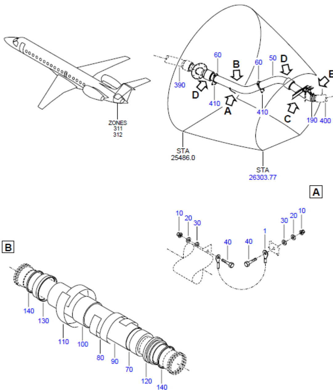
FIGURE 10A(SUP) - ENGINE BLEED AIR SYS INSTL, BTW FR 76 AND FR 80 Sheet 1 of 2
