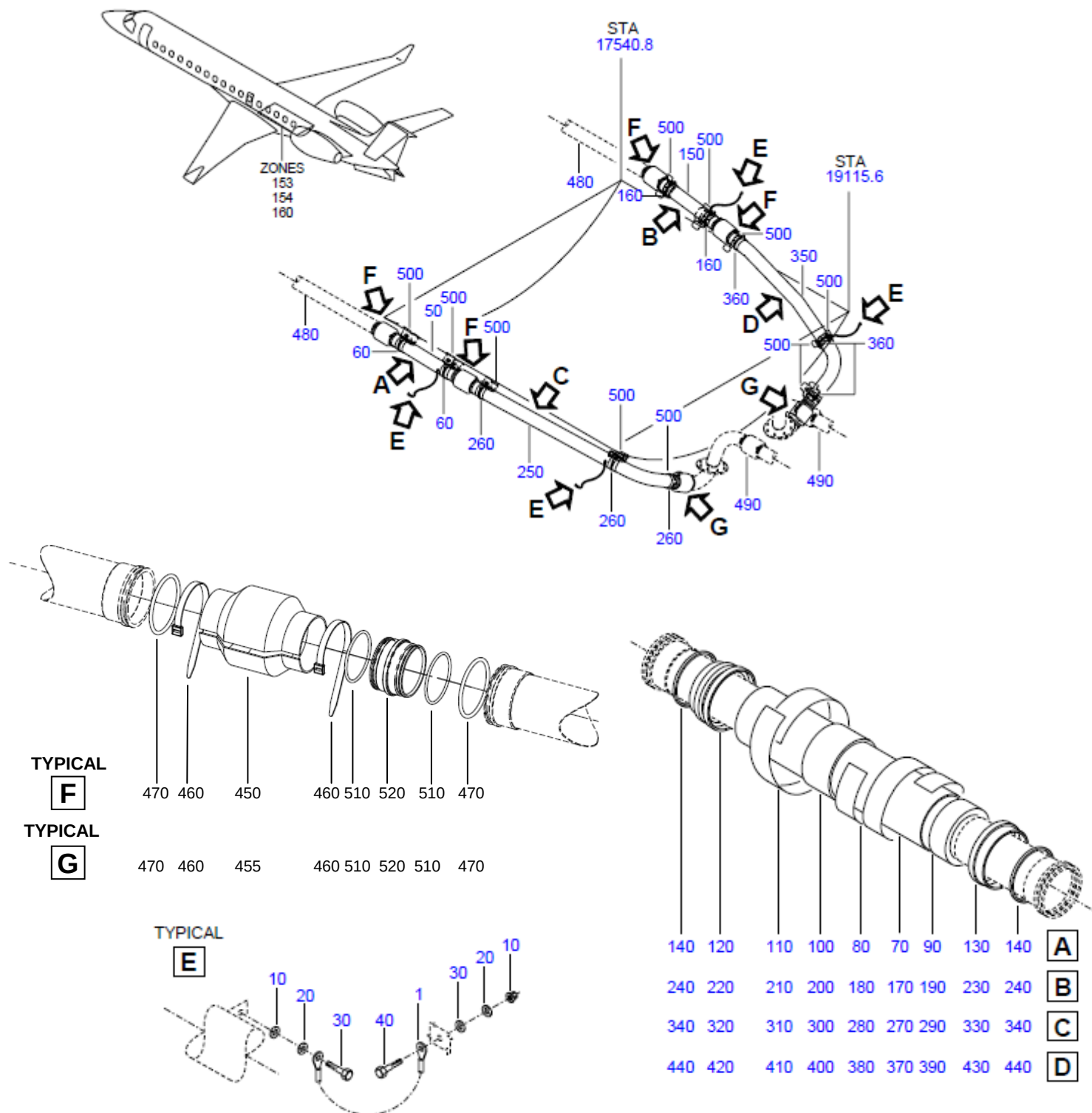
FIGURE 01(SUP) - ENGINE BLEED AIR SYS INSTL, BTW FR 52 AND FR 56
