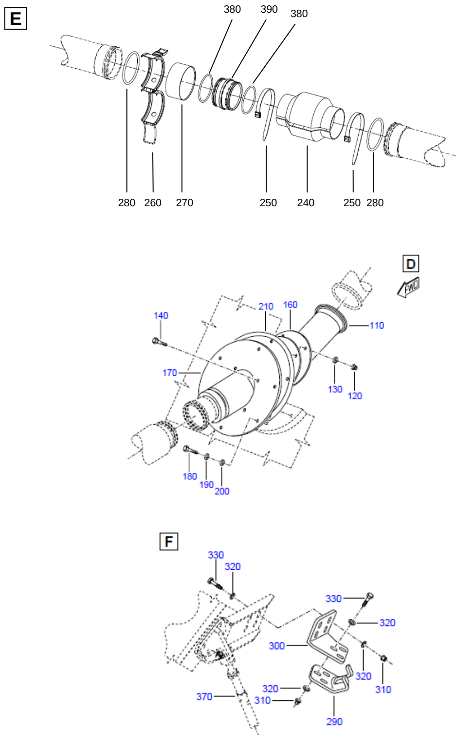
FIGURE 11A(SUP) - ENGINE BLEED AIR SYS INSTL, BTW FR 76 AND FR 80 Sheet 2 of 2
