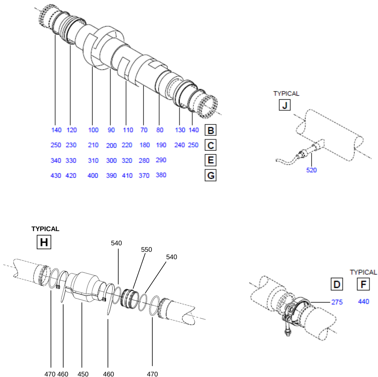
FIGURE 01(SUP) - ENGINE BLEED AIR SYS INSTL, BTW 60 AND FR 70 Sheet 2 of 2
