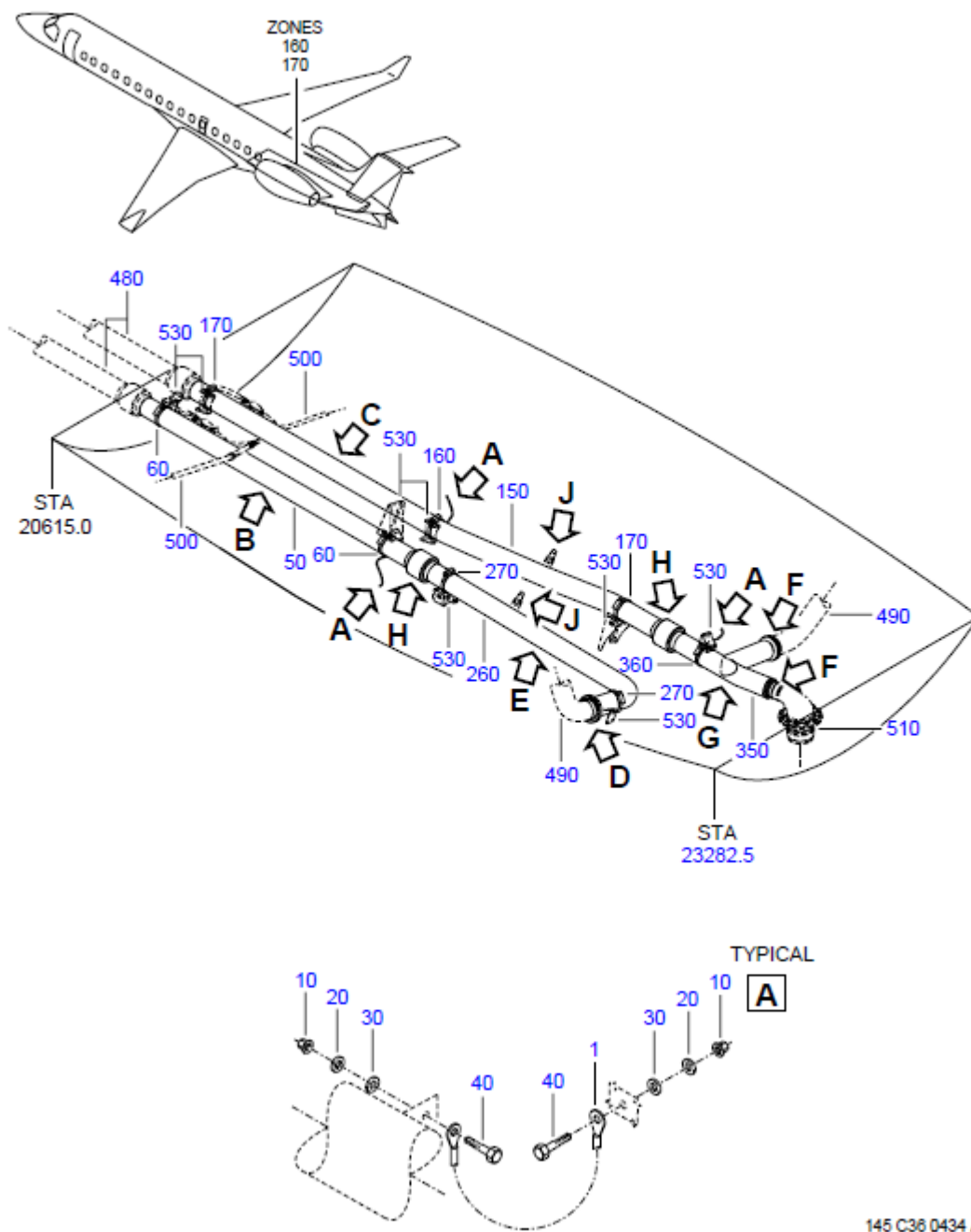
FIGURE 01(SUP) - ENGINE BLEED AIR SYS INSTL, BTW FR 60 AND FR 70 Sheet 1 of 2
