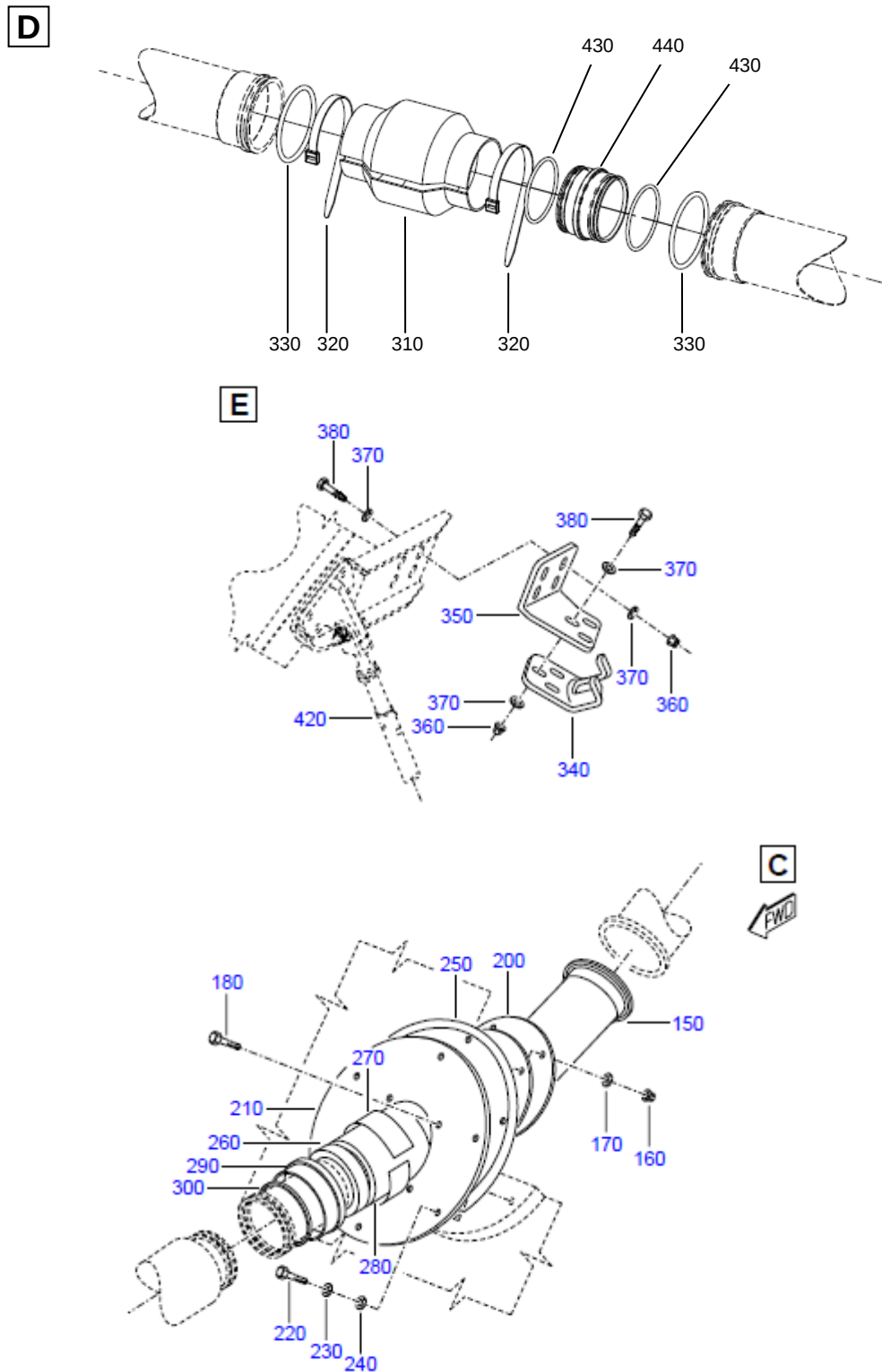
FIGURE 10A(SUP) - ENGINE BLEED AIR SYS INSTL, BTW FR 76 AND FR 80 Sheet 2 of 2
