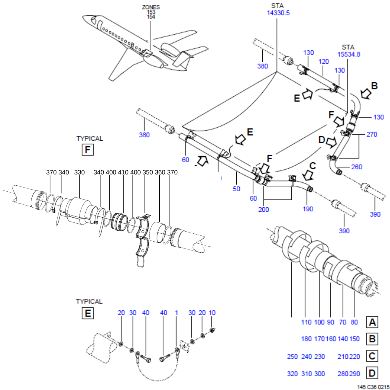
FIGURE 22(SUP) - ENGINE BLEED AIR SYS INSTL, BTW FR 49 AND FR 52
