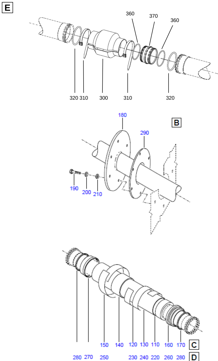
FIGURE 01(SUP) - ENGINE BLEED AIR SYS INSTL, BTW FR 74 AND FR 76 Sheet 2 of 2
