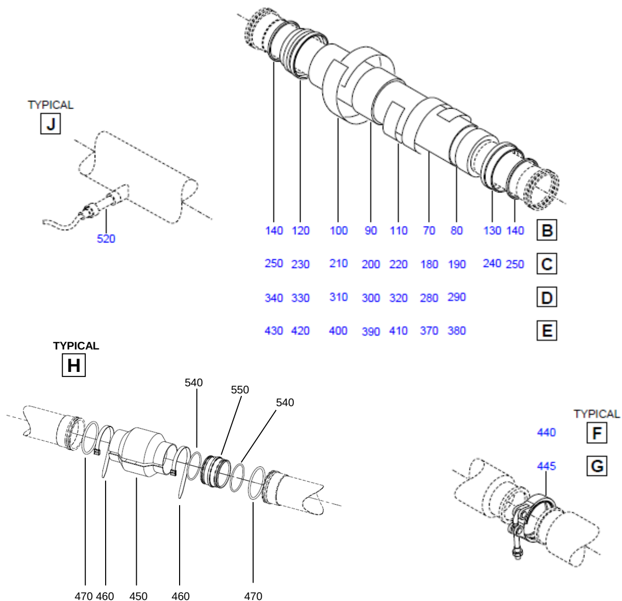
FIGURE 03(SUP) - ENGINE BLEED AIR SYS INSTL, BTW FR 60 AND FR 70 Sheet 2 of 2
