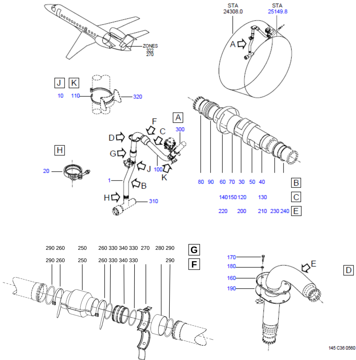
FIGURE 22(SUP) - ENGINE BLEED AIR SYS INSTL, BTW FR 73 AND FR 75
