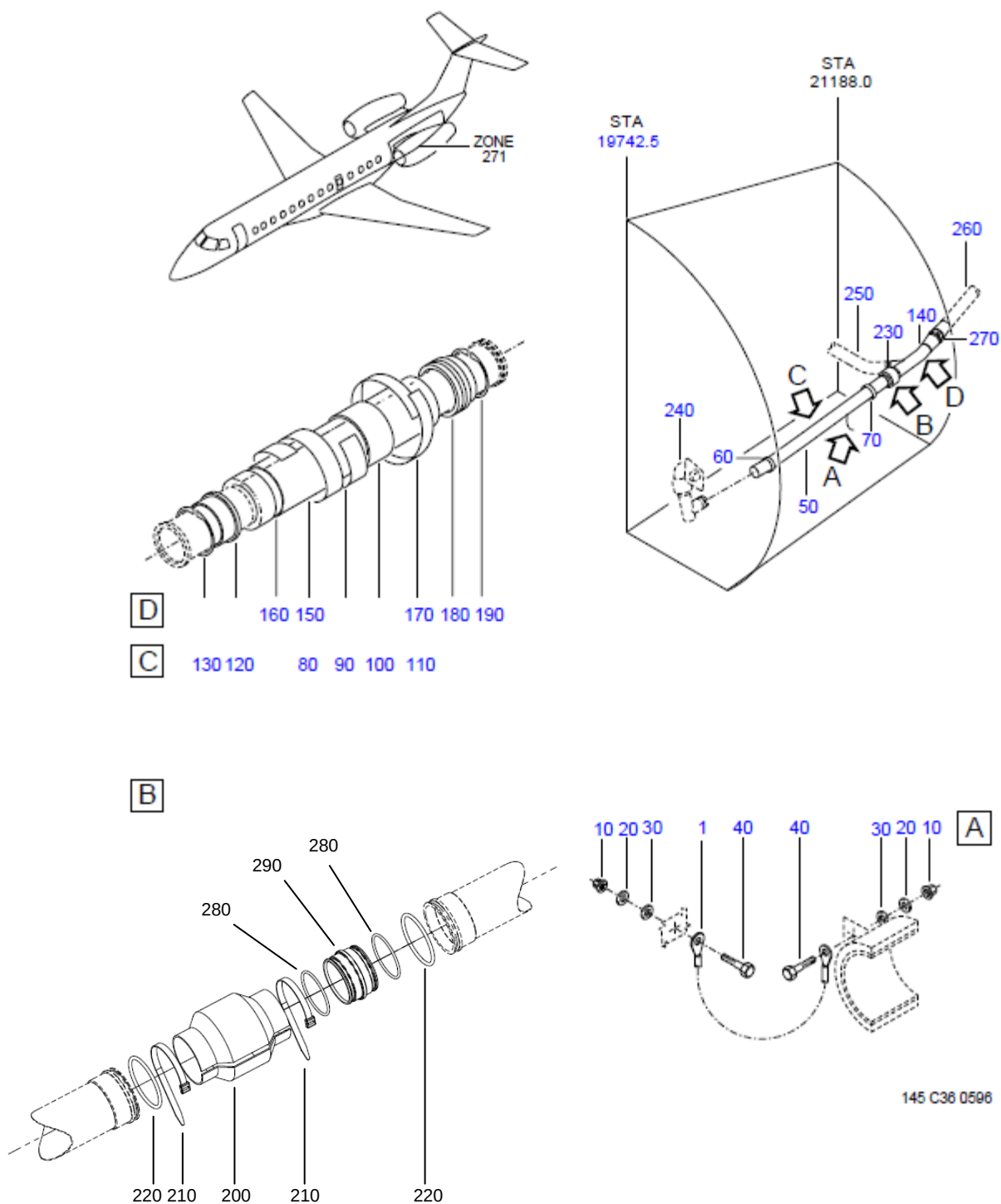
FIGURE 42(SUP) - ENGINE BLEED AIR SYS INSTL, BTW FR 70 AND FR 74, LH SIDE
