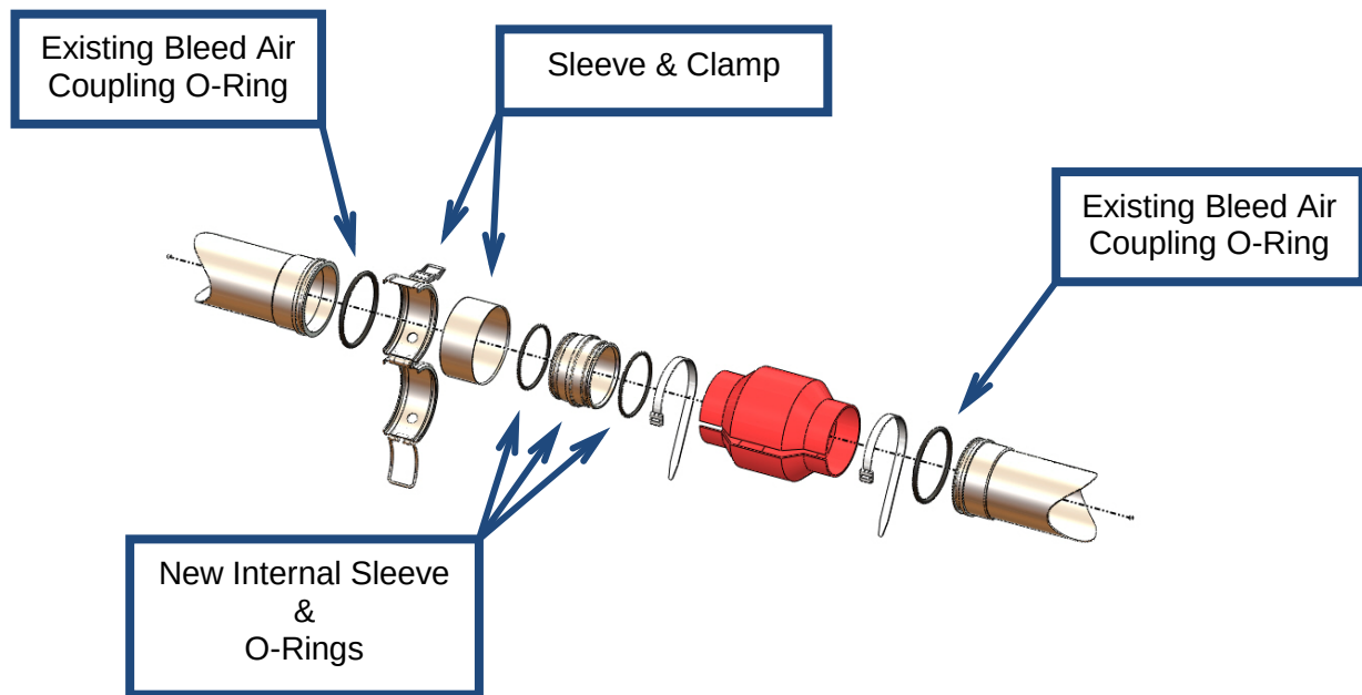
Figure 2 Bleed Air Duct Coupling Flanged Design with External Sleeve & Clamp
