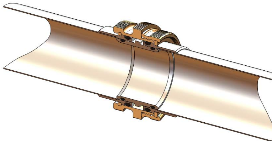
Figure 3 Assembled Bleed Air Duct Coupling Flanged Design with Threaded Coupler & Retaining Nut Cross Sectioned View
