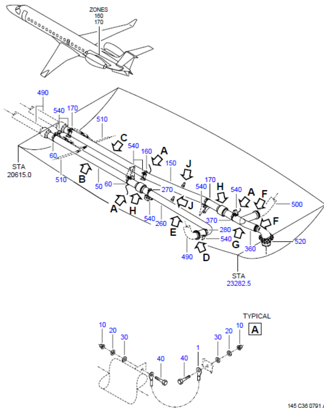
FIGURE 02(SUP) - ENGINE BLEED AIR SYS INSTL, BTW FR 60 AND FR 70 Sheet 1 of 2
