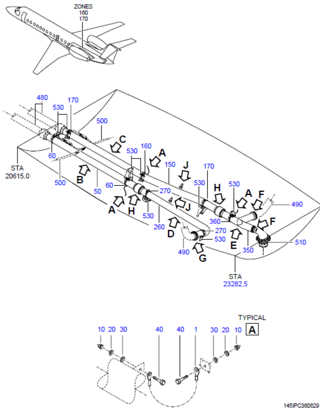
FIGURE 03(SUP) - ENGINE BLEED AIR SYS INSTL, BTW FR 60 AND FR 70 Sheet 1 of 2
